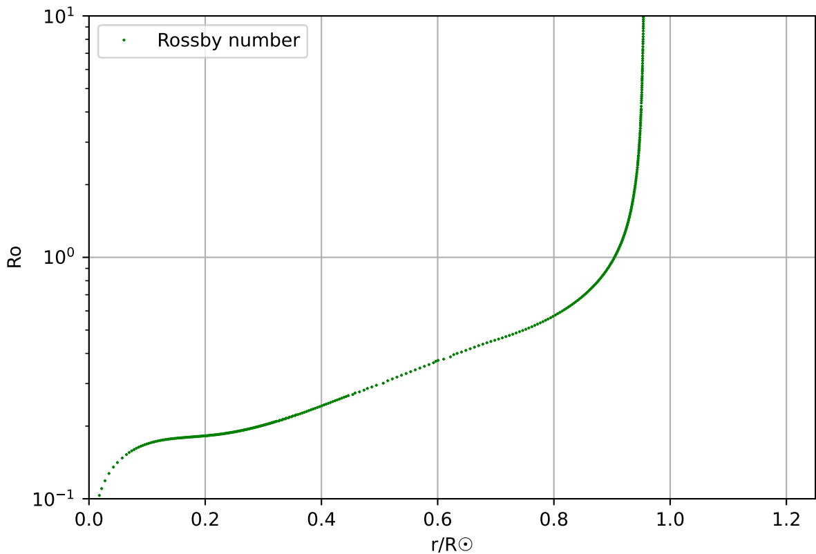
Rossby number, profile 141, age 3.21 \times 10^9
